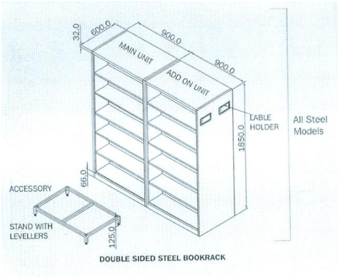
Figure 1: Double Sided Book Rack
